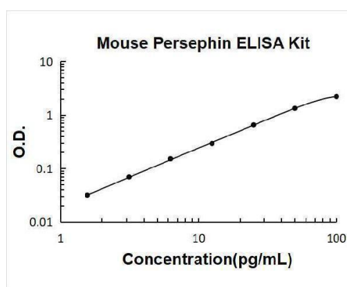
Mouse Persephin ELISA Kit standard curve
