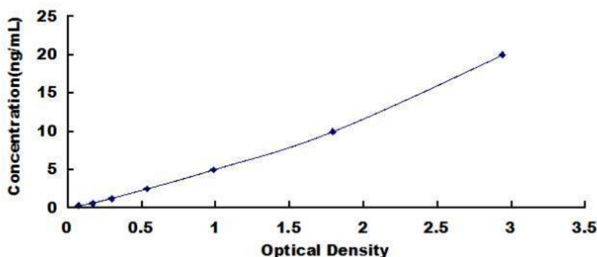
Typical Standard Curve for Human GDA ELISA
