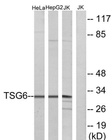
Western blot analysis of lysates from Jurkat, HeLa, and HepG2 cells, using TSG6 Antibody. The lane on the right is blocked with the synthesized peptide.
