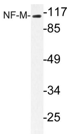
Western blot analysis of lysate from MCF-7 cells, using NF-M antibody.
