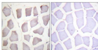
Immunohistochemistry analysis of paraffin-embedded human skeletal muscle, using CRYAB/Crystallin-alpha-B (Phospho-Ser59) Antibody. The picture on the right is blocked with the phosphopeptide.
