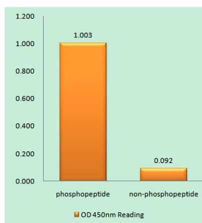
Enzyme-Linked Immunosorbent Assay (Phospho-ELISA) for Immunogen Phosphopeptide (Phospho-left) and Non-Phosphopeptide (Phospho-right), using Chk1 (Phospho-Ser286) Antibody
