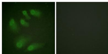
Immunofluorescence analysis of HeLa cells, using Chk1 (Phospho-Ser286) Antibody. The picture on the right is blocked with the phospho peptide.
