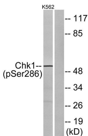
Western blot analysis of lysates from K562 cells treated with Na3VO4 0.3uM 40', using Chk1 (Phospho-Ser286) Antibody. The lane on the right is blocked with the phospho peptide.
