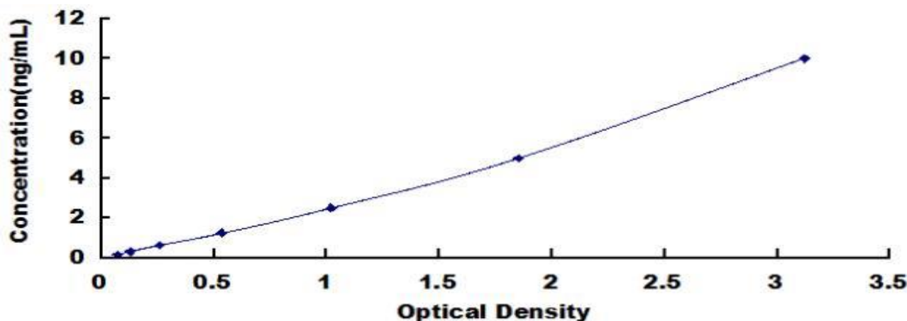
Typical Standard Curve for Rat IL11Ra ELISA.
