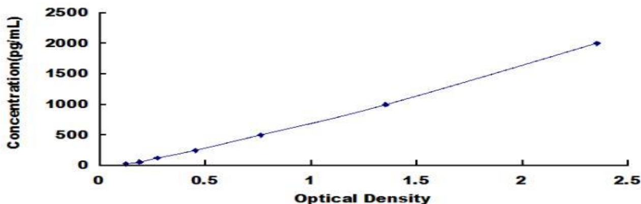
Typical Standard Curve for Rat HMG1 ELISA.
