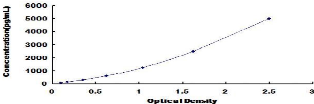
Typical Standard Curve for Rat GROg ELISA.
