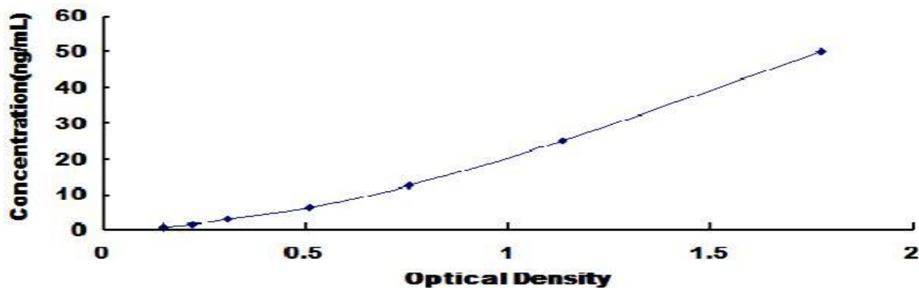
Typical Standard Curve for Rat GSS ELISA.
