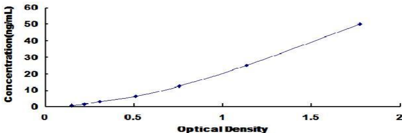
Typical Standard Curve for Rat ENG ELISA.
