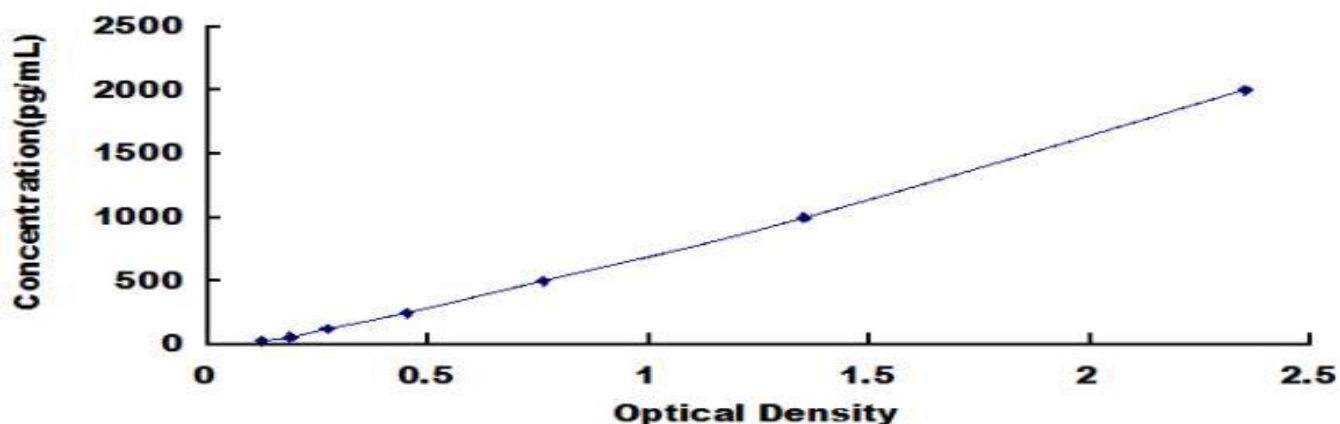
Typical Standard Curve for Rat EG-VEGF ELISA.
