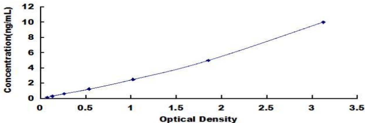
Typical Standard Curve for Rat DUOX2 ELISA.
