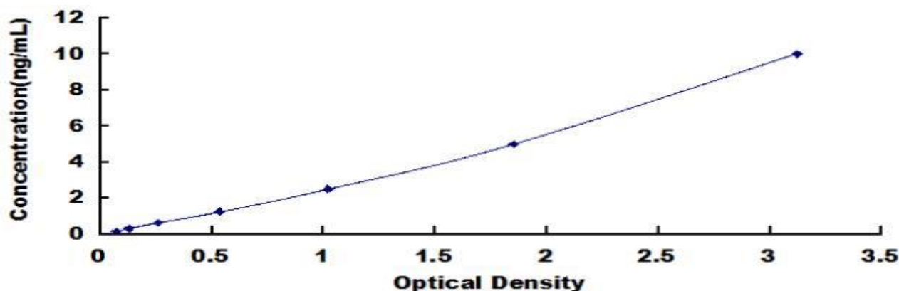
Typical Standard Curve for Rat DEFb2 ELISA.
