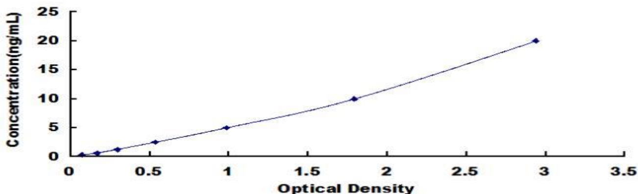
Typical Standard Curve for Rat CYP1A1 ELISA.
