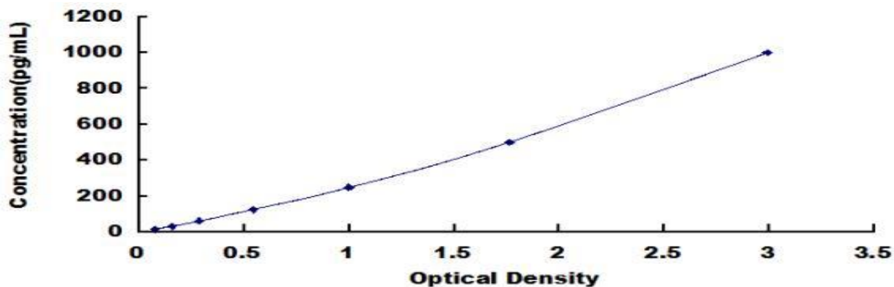
Typical Standard Curve for Rat CRHBP ELISA.
