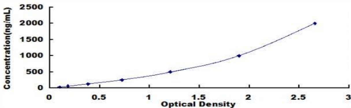
Typical Standard Curve for Rat CFB ELISA.
