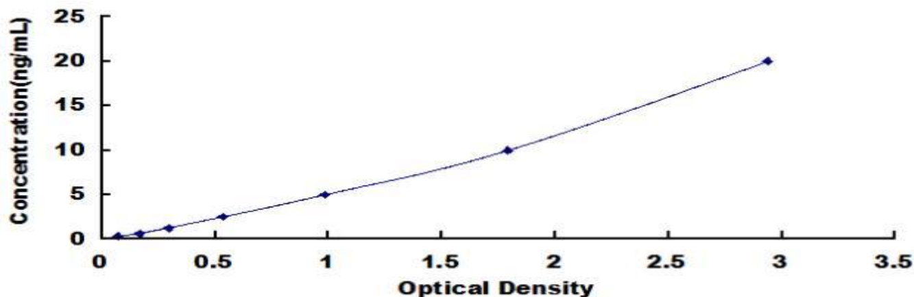
Typical Standard Curve for Rat CHRNa1 ELISA.
