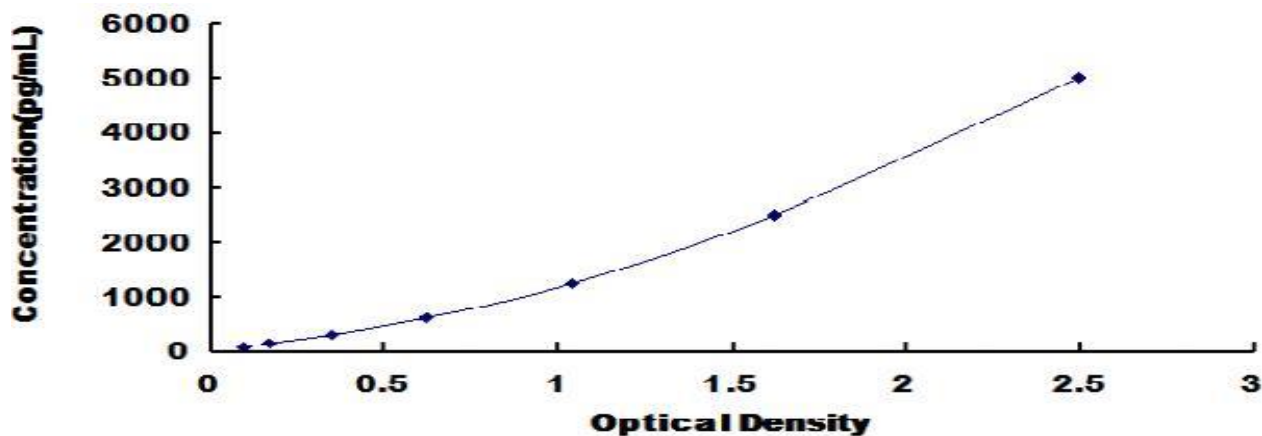
Typical Standard Curve for Mouse TIMP4 ELISA.
