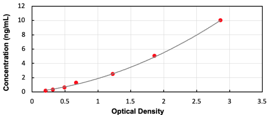
Typical Standard Curve for Human ATP1b3 ELISA
