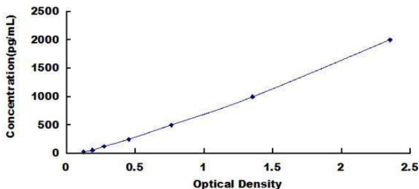
Typical Standard Curve for Human CGRP1 ELISA
