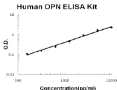
Human OPN PicoKine ELISA Kit standard curve
