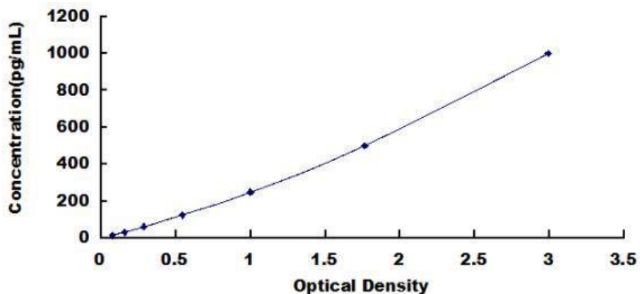
Typical Standard Curve for Human SNcα ELISA.
