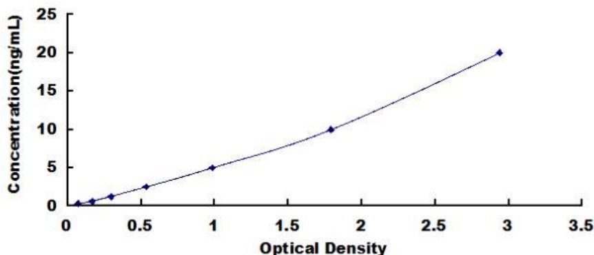
Typical Standard Curve for Rat SDF1 ELISA.
