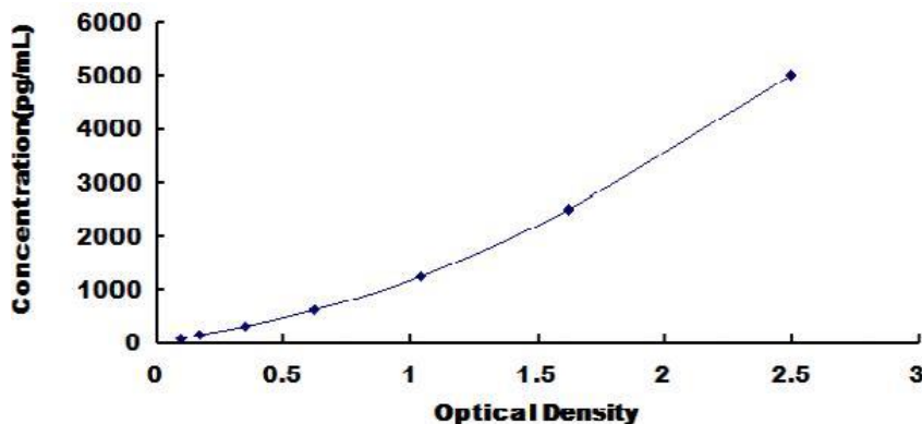
Typical Standard Curve for Bovine RANTES ELISA.
