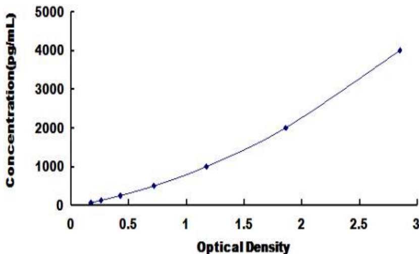
Typical Standard Curve for Human HMG1 ELISA.
