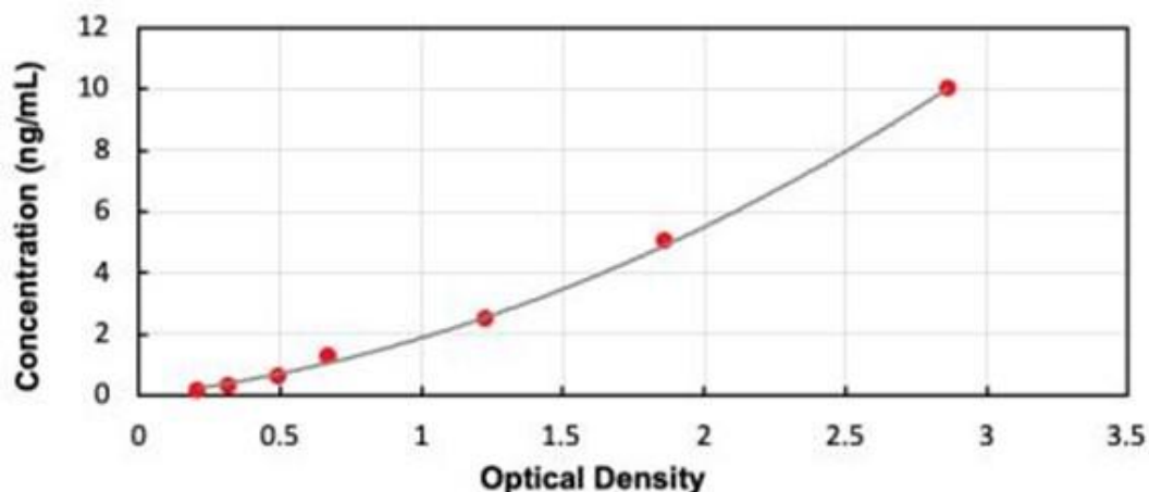
Typical Standard Curve for Human EN2 ELISA
