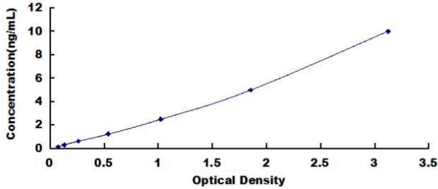
Typical Standard Curve for Rabbit CRP ELISA.
