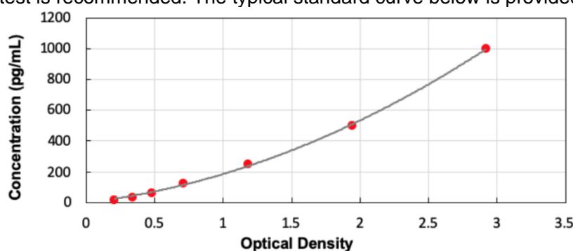
Typical Standard Curve for Human ADM ELISA
