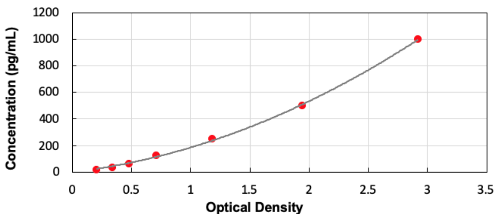
Typical Standard Curve for Human ACE2 ELISA
