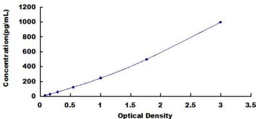
Typical Standard Curve for Human VEGFD ELISA.
