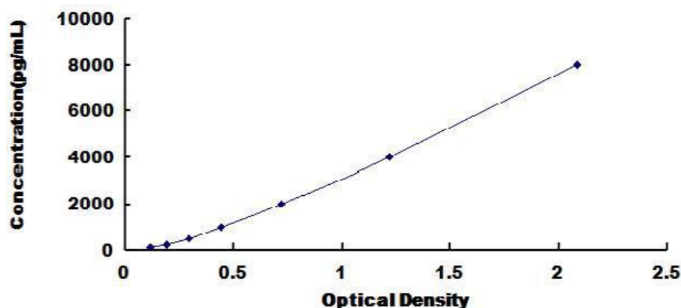
Typical Standard Curve for Bovine NGF ELISA.
