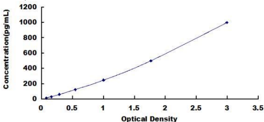
Typical Standard Curve for Equine IL1b ELISA.
