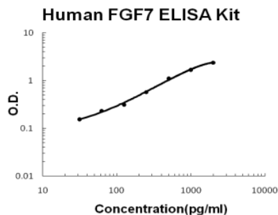
Human FGF7/KGF ELISA Kit standard curve
