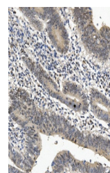
IHC analysis of EYA4 using anti-EYA4 ant...
