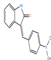
Chemical structure of SU4312.
