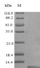
SDS-PAGE analysis of Human NRG1 protein ...
