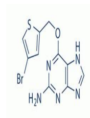
Lomeguatrib (PaTrin-2)
