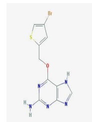
Chemical structure of Lomeguatrib (PaTri...
