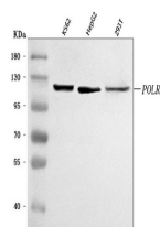
WB analysis of POLR1B using anti-POLR1B ...
