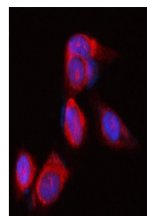
IF analysis of POLR1B using anti-POLR1B ...
