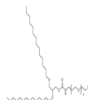
Chemical Structure (1019000-64-6)
