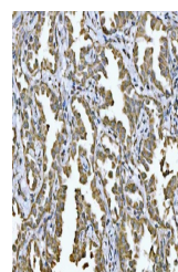
IHC analysis of NDUFV2 using anti-NDUFV2...
