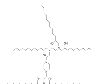
Chemical structure of orb1146680
