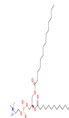
CAS Number: 18194-24-6
