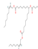
Chemical structure of orb1089401
