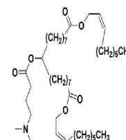
Chemical structure of orb1089401
